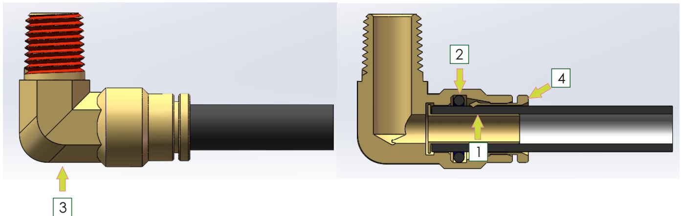
1 Tube support/Insert 2 'O' -ring 3 Body 4 Pipe clamp
